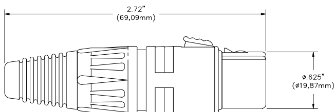
Model 7283, 3-Pin (M) In-Line XLR, Silver Contacts, Nickel Finish
